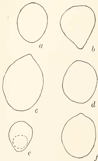
FIG. 2. Camera-lucida outlines showing variations in size. Figure e vacuolated. (See text for explanation.) Magnification 1825 X.
